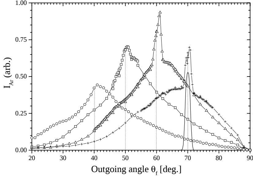
Figure 6.4: Angular distribution of Ar scattered from the Ru(0001)-(1 \times 1)H surface. E_i=65\text{meV} , T_s=140\text{ K} , \theta_i=40^\circ (circles), 50^\circ (squares), 60^\circ (triangles) and 70^\circ (crosses) along the close packed \langle 11\bar{2}0 \rangle direction. Angular profile of the direct beam ( 70^\circ ) is shown for comparison.
