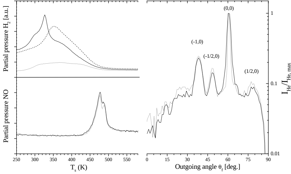
Figure 6.3: Left panel: TPD spectra of H_2 and NO from Ru(0001)-(1x1)H (dashed lines); Ru(0001)-(2x2)NO (dotted lines) and Ru(0001)-(1x1)H exposed to an NO beam (solid lines). Heating rate 5\text{ Ks}^{-1} . Right panel: Normalized scattered helium intensity from Ru(0001)-(2x2)NO and Ru(0001)-(1x1)H + NO, E_i = 65\text{ meV} , \theta_i = 60^\circ along the close packed \langle 11\bar{2}0 \rangle direction, T_s = 140\text{ K} . Labels show diffraction peak indices.
